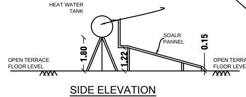
SIDE ELEVATION
