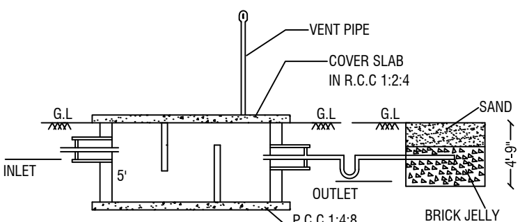
SECTION-AB
