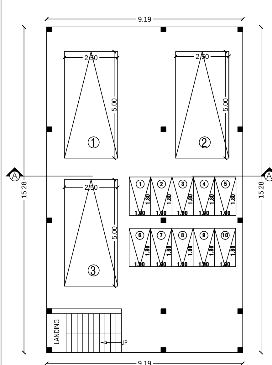
STILT FLOOR
