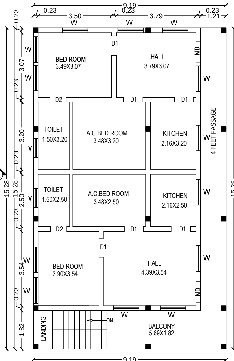
THIRD FLOOR
