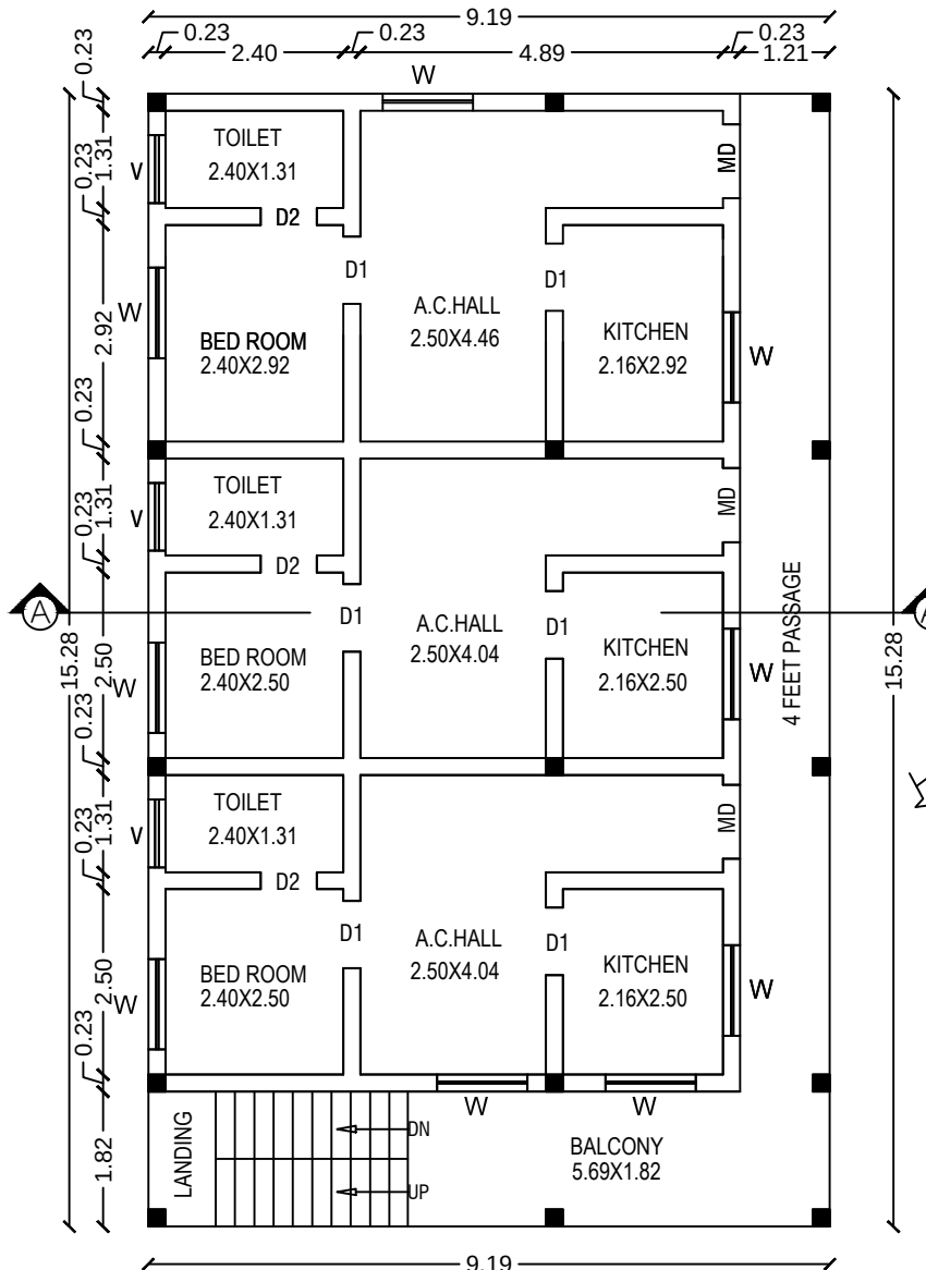
FIRST FLOOR
