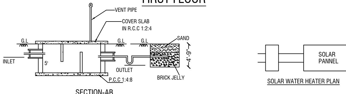
SECTION-AB
