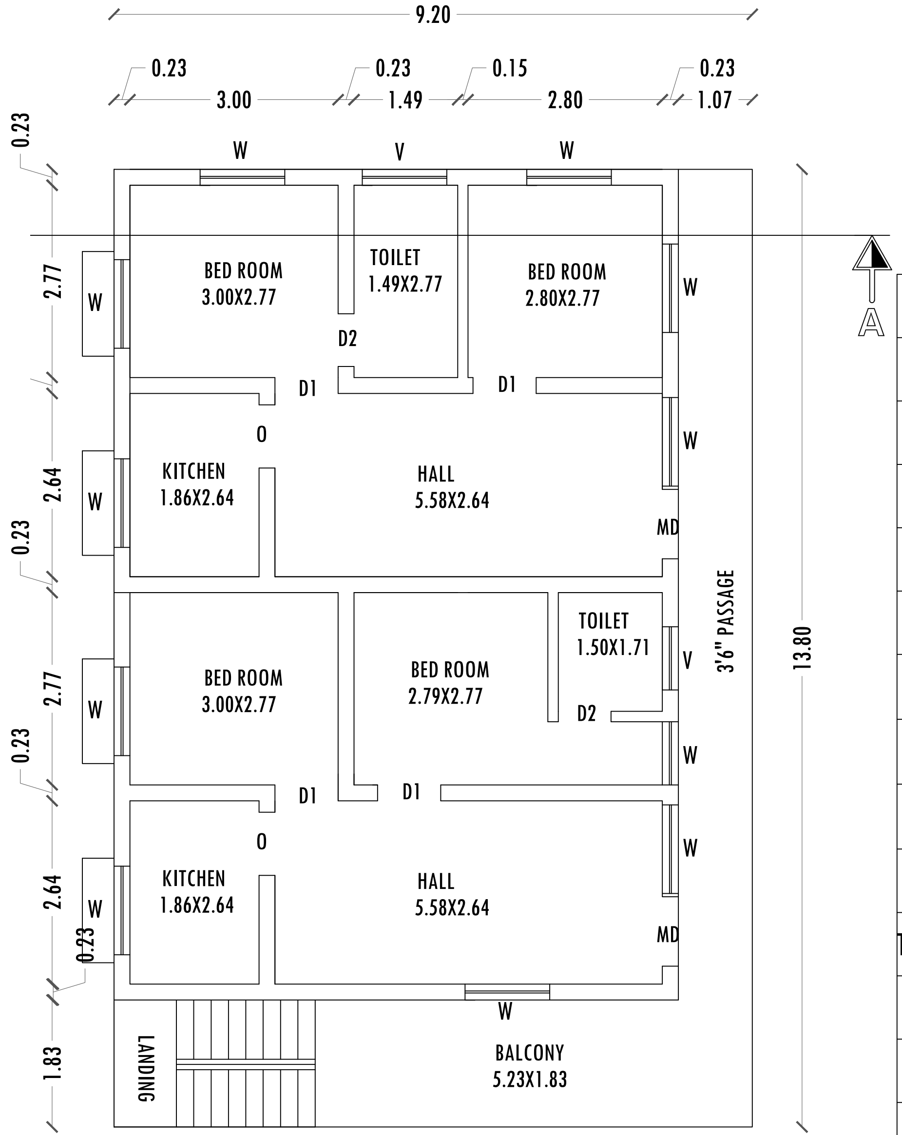
SECOUND FLOOR PLAN
