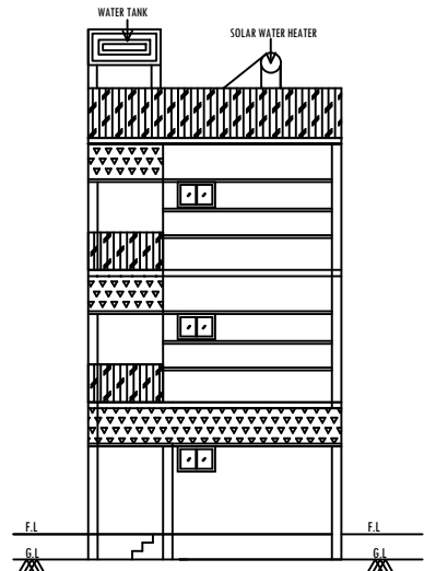
WEST SIDE ELEVATION
