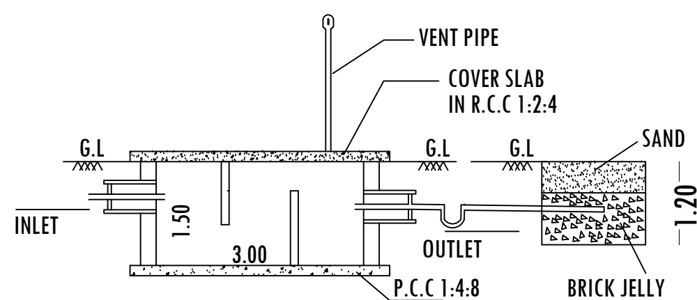
SECTION-AB
