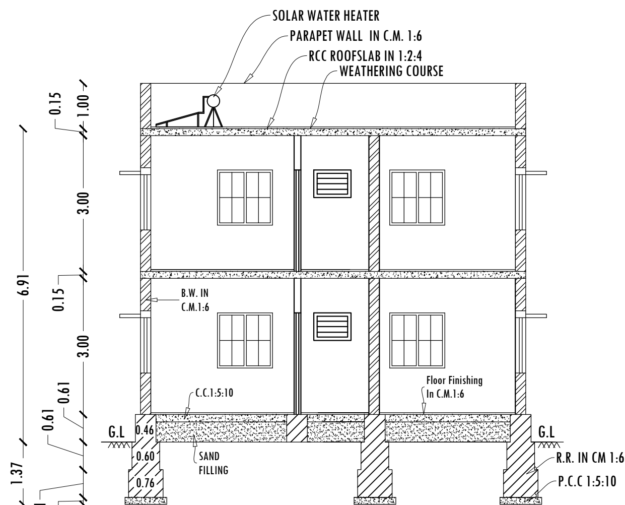
SECTION-AA
