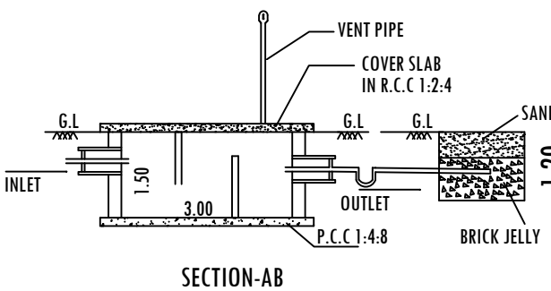
SECTION-AB
