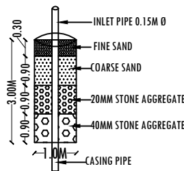
DETAILS OF RAIN WATER
