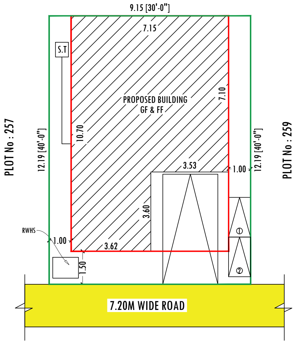
SITE PLAN
