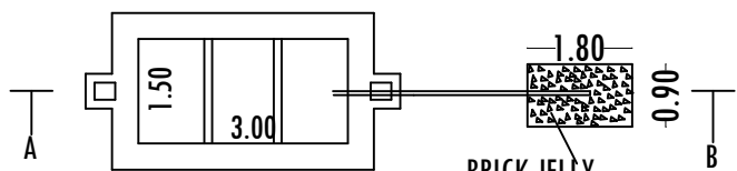
SEPTIC TANK & DISPERSION TRENCH DETAILS
