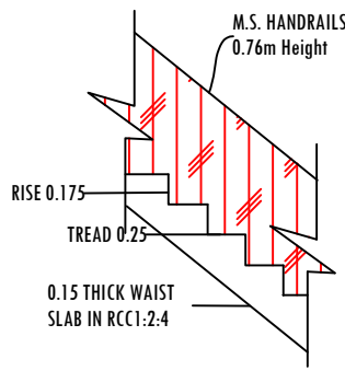
STAIRCASE DETAILS
