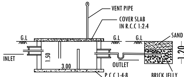
SECTION-AB
