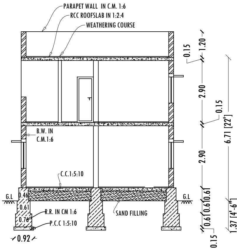
SECTION -AA
