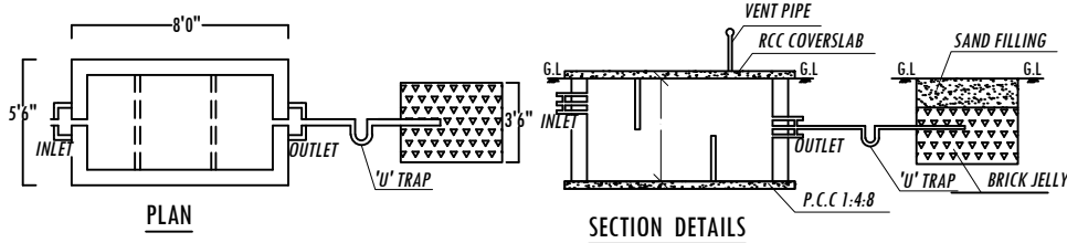
SEPTIC TANK AND DISPERSION TRENCH DETAILS
