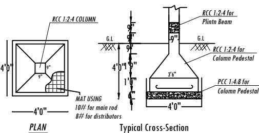
Typical Cross-Section
