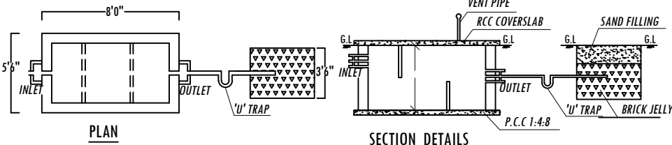
SEPTIC TANK AND DISPERSION TRENCH DETAILS
