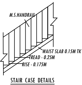
STAIR CASE DETAILS
