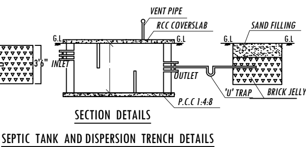
SEPTIC TANK AND DISPERSION TRENCH DETAILS
