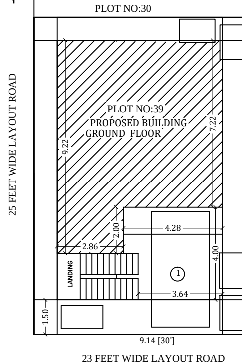
SITE PLAN
