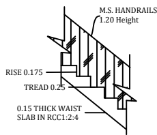
STAIRCASE DETAILS SCALE-1:20
