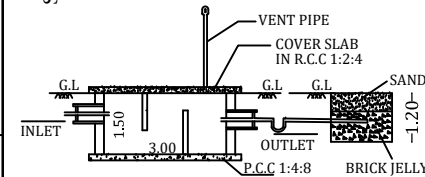
SECTION-AB
