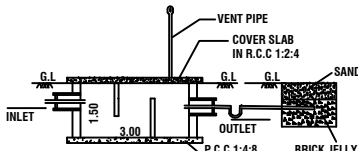
SECTION-AB
