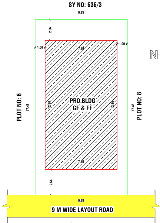
SITE PLAN
