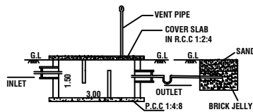
SECTION-AB
