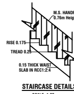
STAIRCASE DETAILS
