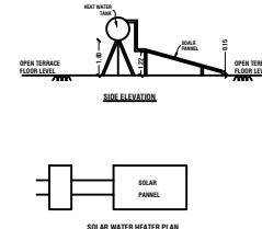
SOLAR WATER HEATER PLAN
