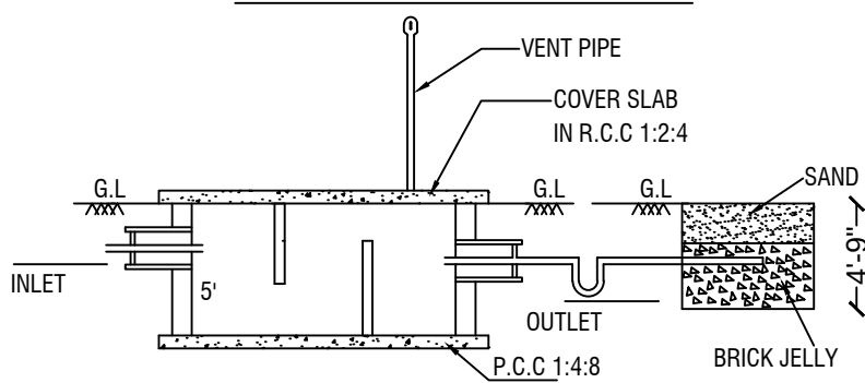
SECTION-AB
