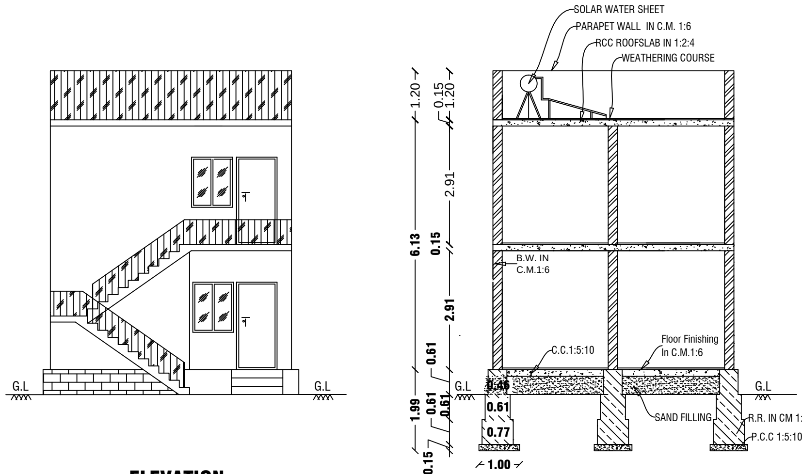
SECTION -AA
