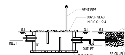
SECTION-AB
