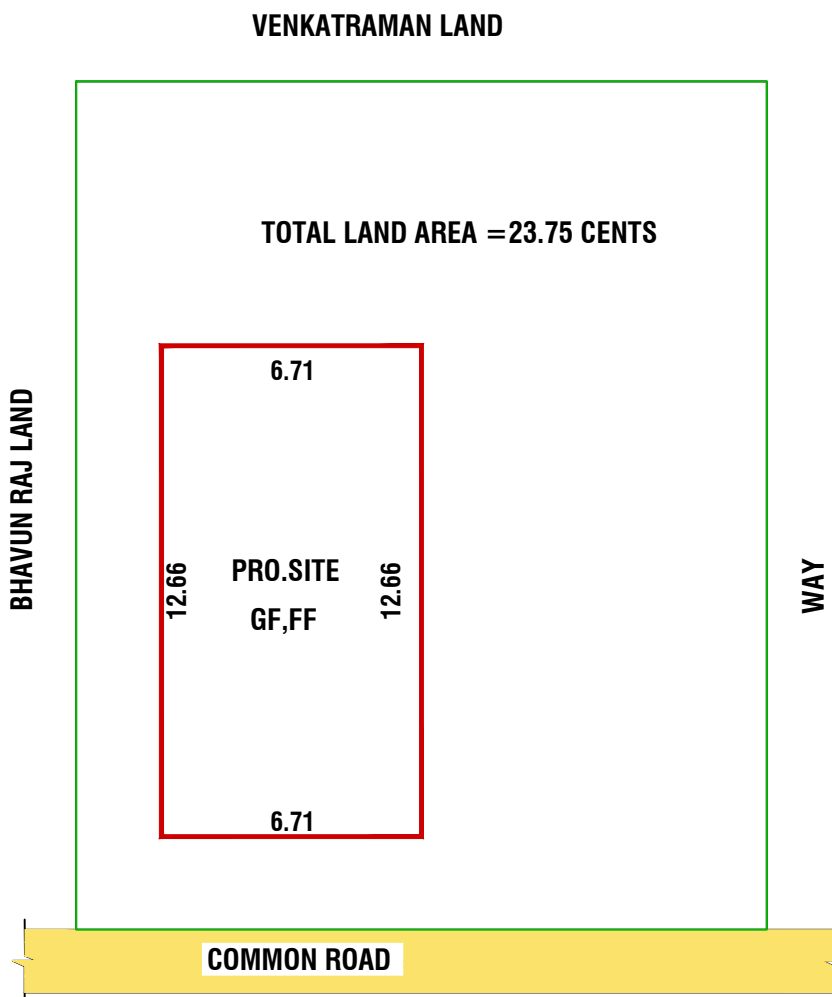
SITE PLAN
