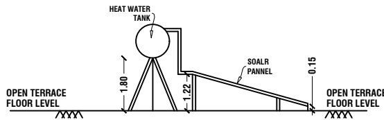
SIDE ELEVATION
