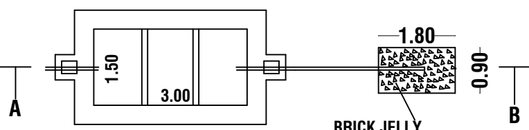
SEPTIC TANK & DISPERSION TRENCH DETAILS
