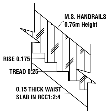
STAIRCASE DETAILS
