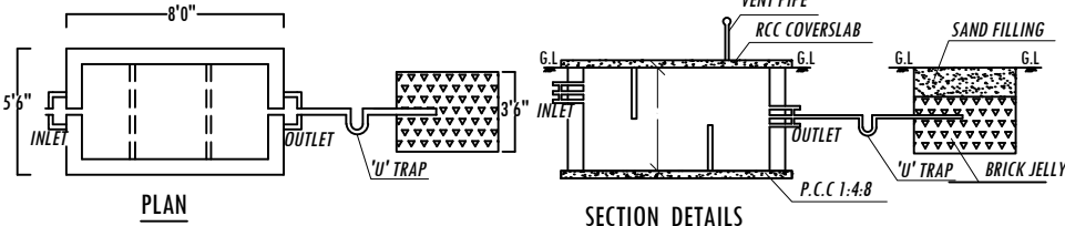
SEPTIC TANK AND DISPERSION TRENCH DETAILS
