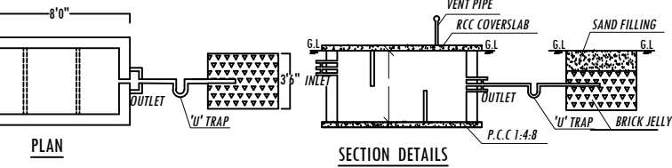
SEPTIC TANK AND DISPERSION TRENCH DETAILS
