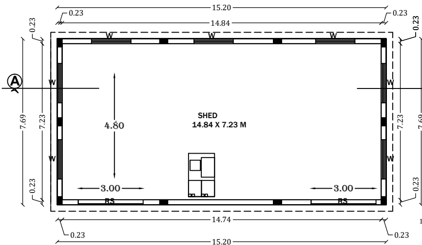
SHED- GROUND FLOOR PLAN
