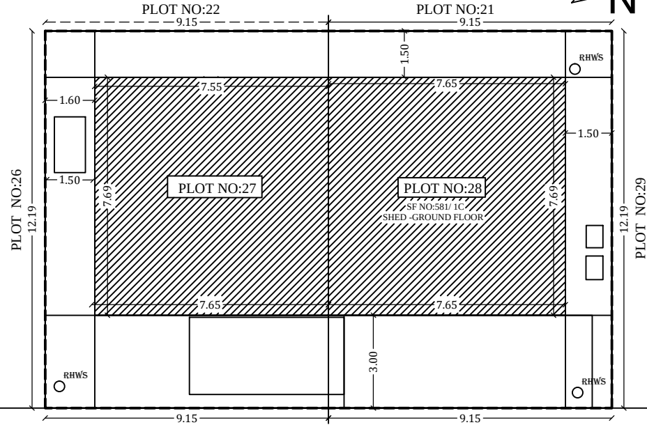
SITE PLAN
