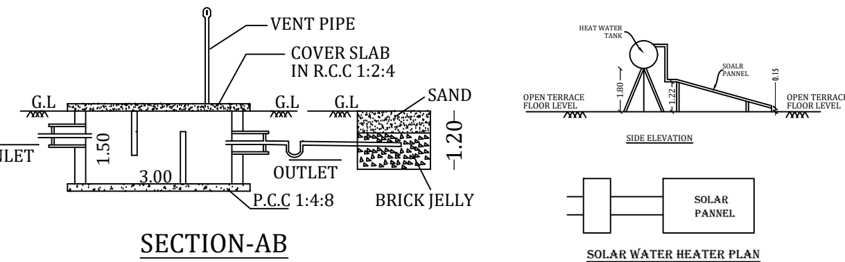
SOLAR WATER HEATER PLAN
