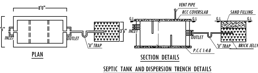
SEPTIC TANK AND DISPERSION TRENCH DETAILS
