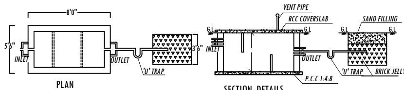
SECTION DETAILS
