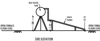
SIDE ELEVATION
