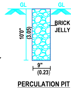
PERCOLATION PIT
