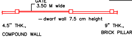
COMPOUND WALL PLAN
