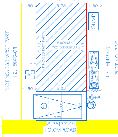
SITE PLAN
