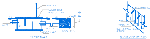
SECTION-AB
