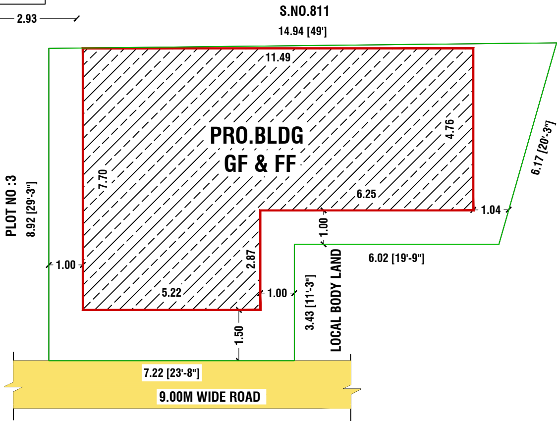
SITE PLAN
