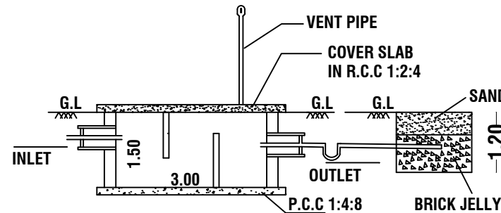
SECTION-AB
