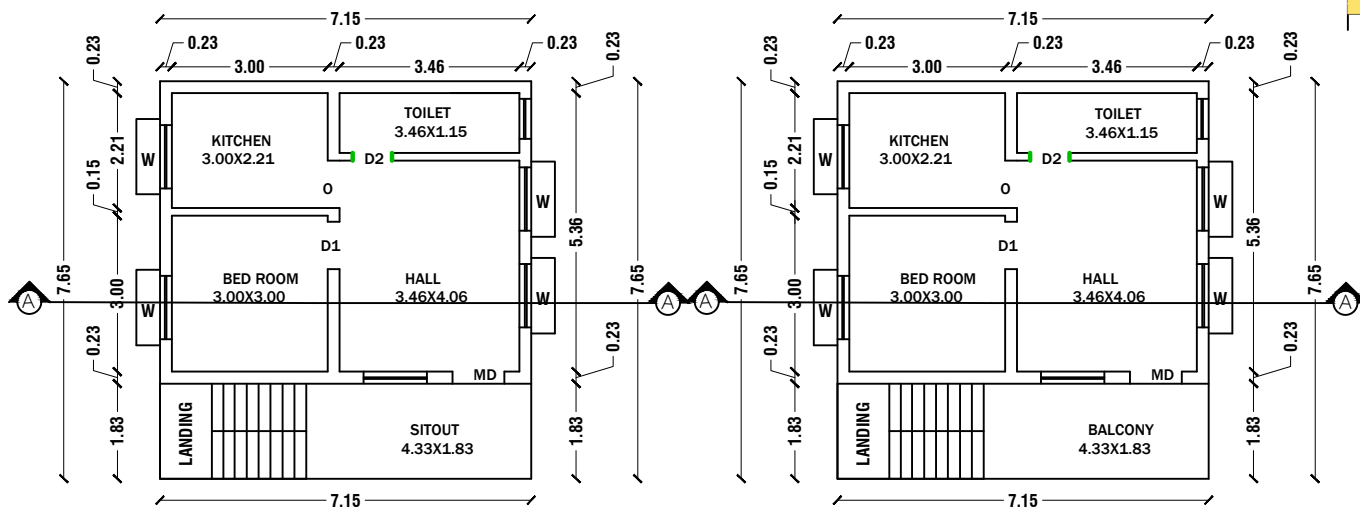
EXT.GROUND FLOOR PLAN
