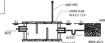
SECTION-AB
