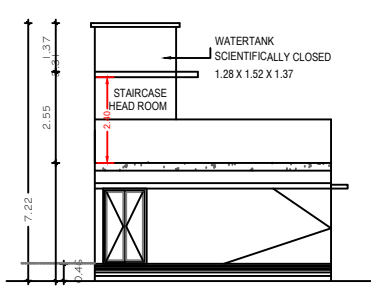
FRONT ELEVATION.
