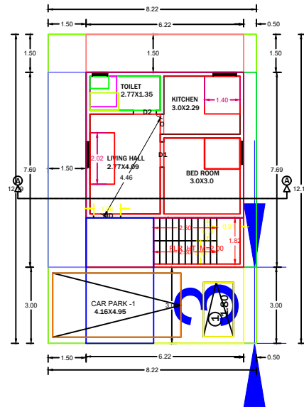
PRO.GROUND FLOOR PLAN SCALE:1:100
