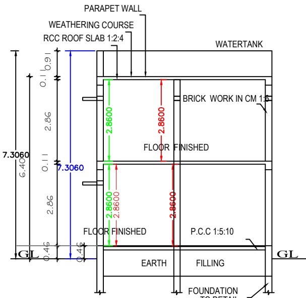
SECTION "A-B"
