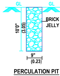
PERCOLATION PIT
