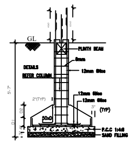
FOUNDATION DETAILS
