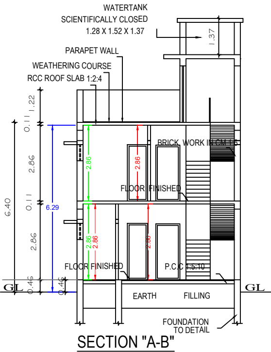
SECTION "A-B"
