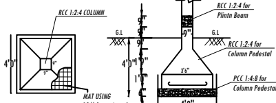
Typical Cross-Section
