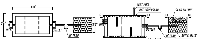
SEPTIC TANK AND DISPERSION TRENCH DETAILS
