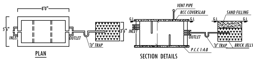
SEPTIC TANK AND DISPERSION TRENCH DETAILS
