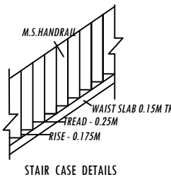
STAIR CASE DETAILS
