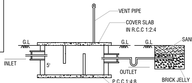
SECTION-AB
