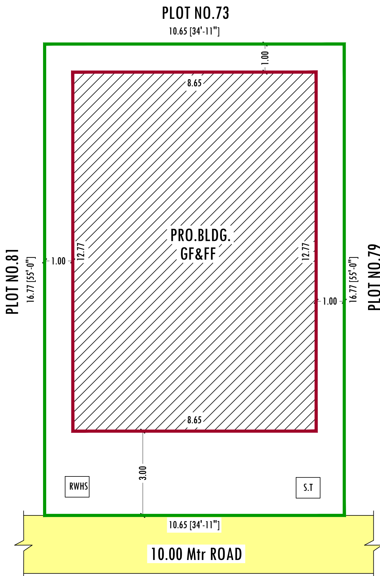
SITE PLAN
