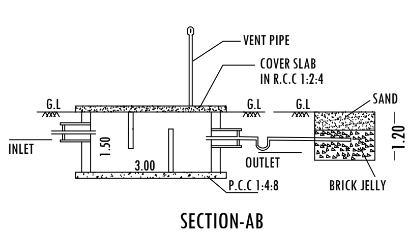
SECTION-AB
