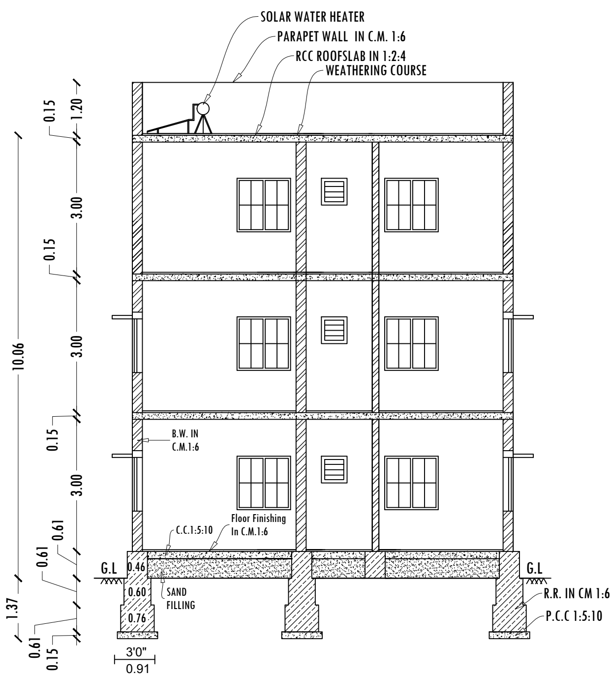
SECTION-AA
