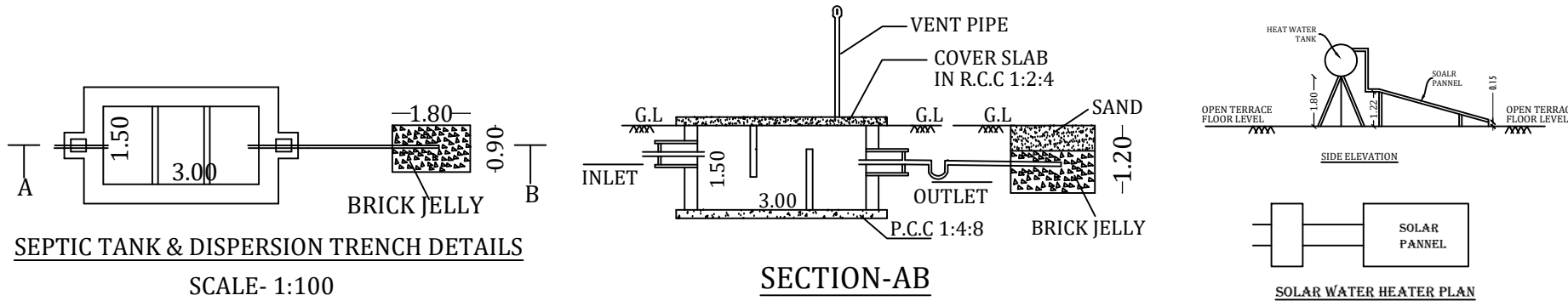
SOLAR WATER HEATER PLAN
