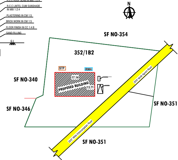
SITE PLAN NOT SCALE
