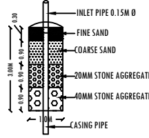
DETAILS OF RAIN WATER HARVESTING STRUCTURES (NOTE TO SCALE)
