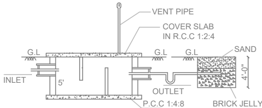
SECTION-AB
