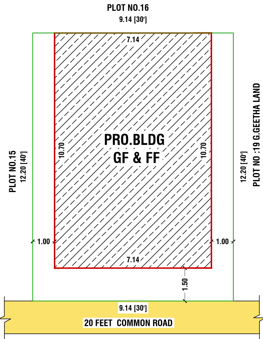
SITE PLAN
