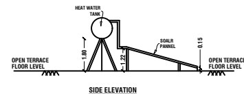
SIDE ELEVATION
