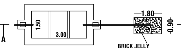
SEPTIC TANK & DISPERSION TRENCH DETAILS SCALE: 1:100
