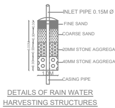
DETAILS OF RAIN WATER HARVESTING STRUCTURES SCALE: 1/20
