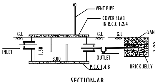
SECTION-AB
