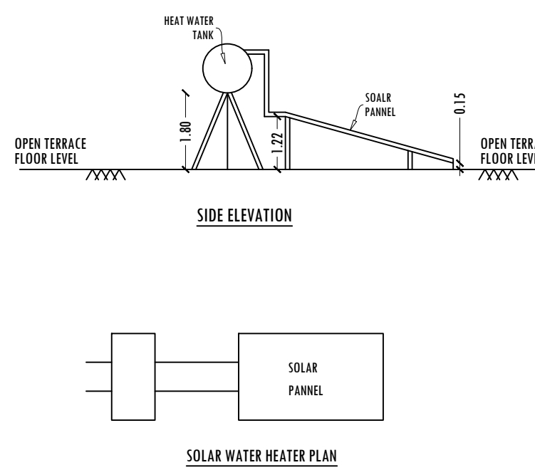
SOLAR WATER HEATER PLAN
