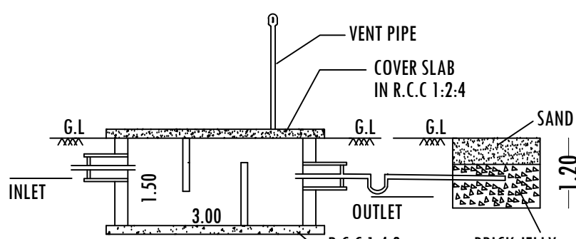
SECTION-AB
