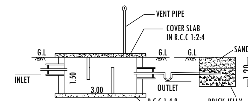
SECTION-AB
