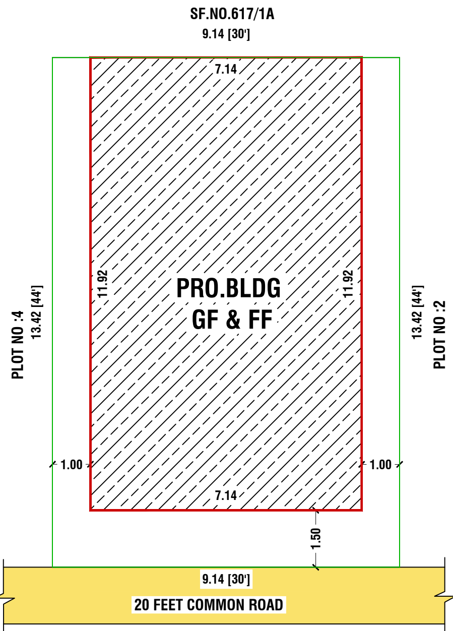
SITE PLAN
