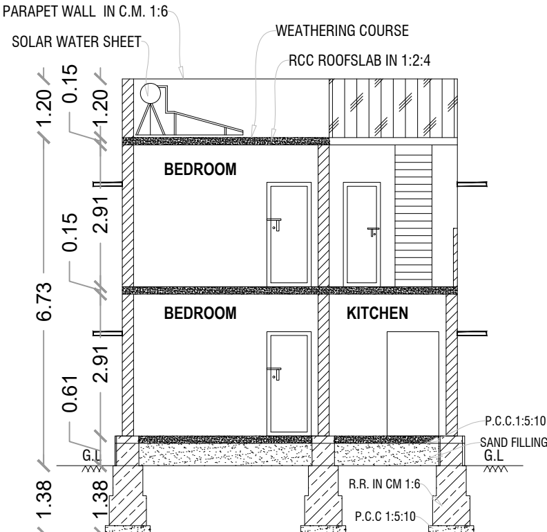
SECTION -AA
