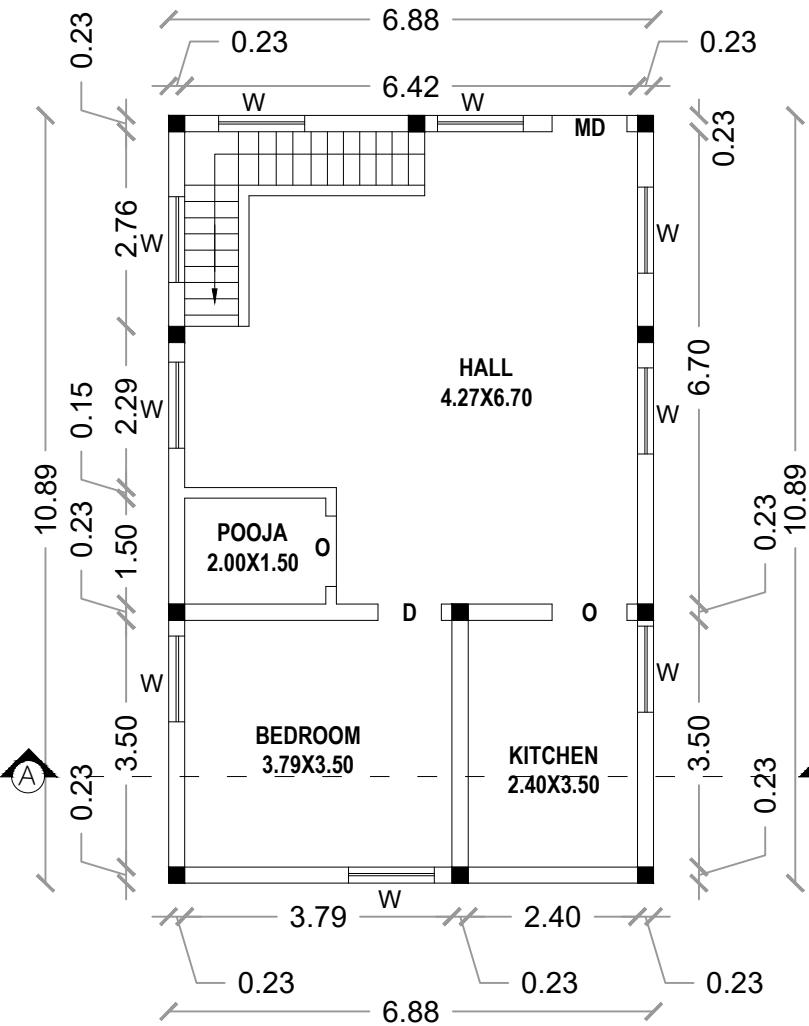
GROUND FLOOR SCALE - 1:100
