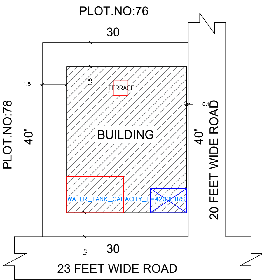
SITE PLAN
