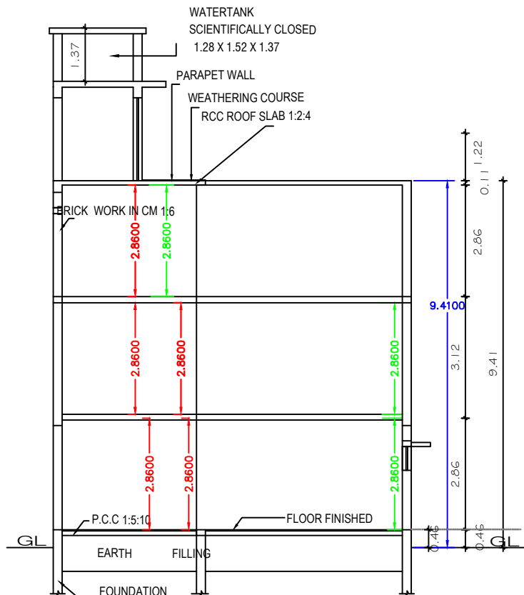
SECTION "A-B"
