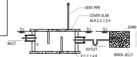
SECTION-AB
