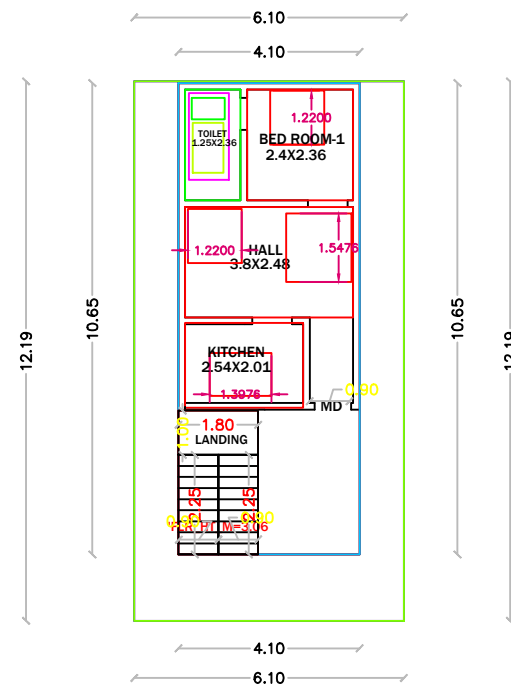
PRO.GROUND FLOOR PLAN SCALE:1:100
