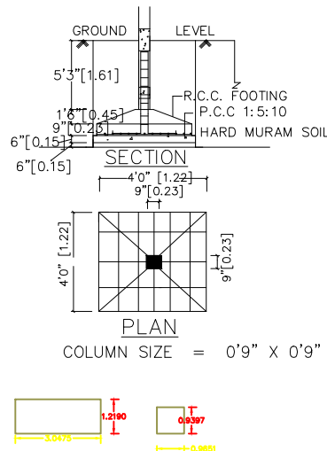
FOUNDATION DETAILS
