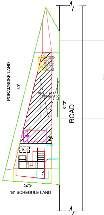
GROUND FLOOR (COMMERCIAL)
