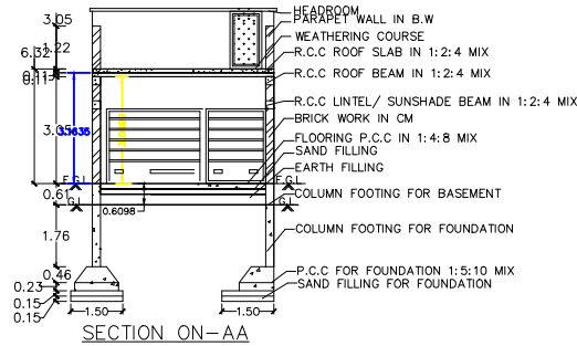
SECTION ON-AA
